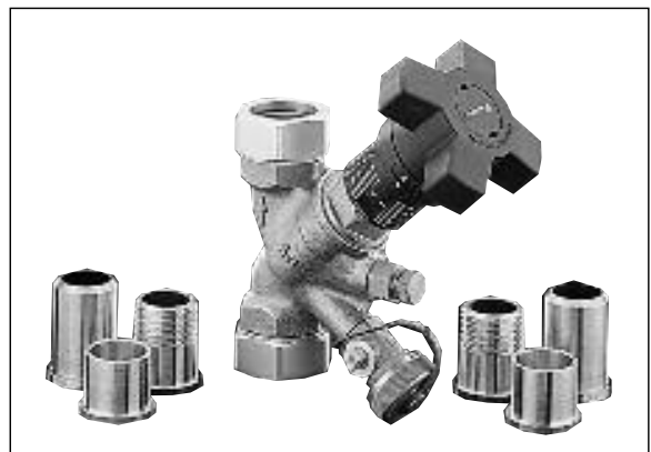
Male threads for weldable steel tailpipes 3/8" to 2" or: ... for solder tailpipes 0.59" x to 1.65" x or: ... for threaded tailpipes 3/8" to 1 1/2"
